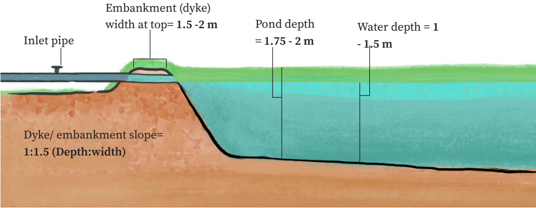
Pond cross-sectional details (inlet side)
