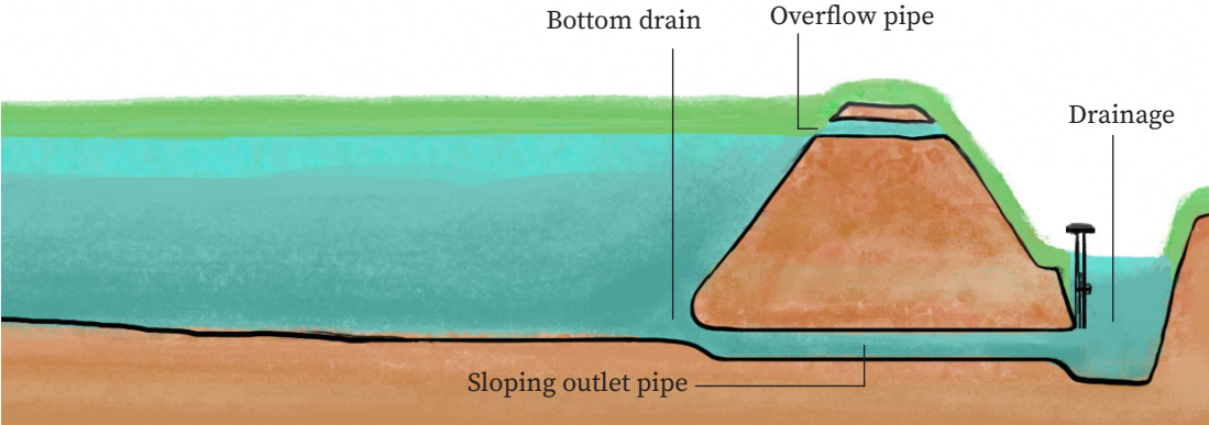
Pond cross-sectional details (outlet side)
